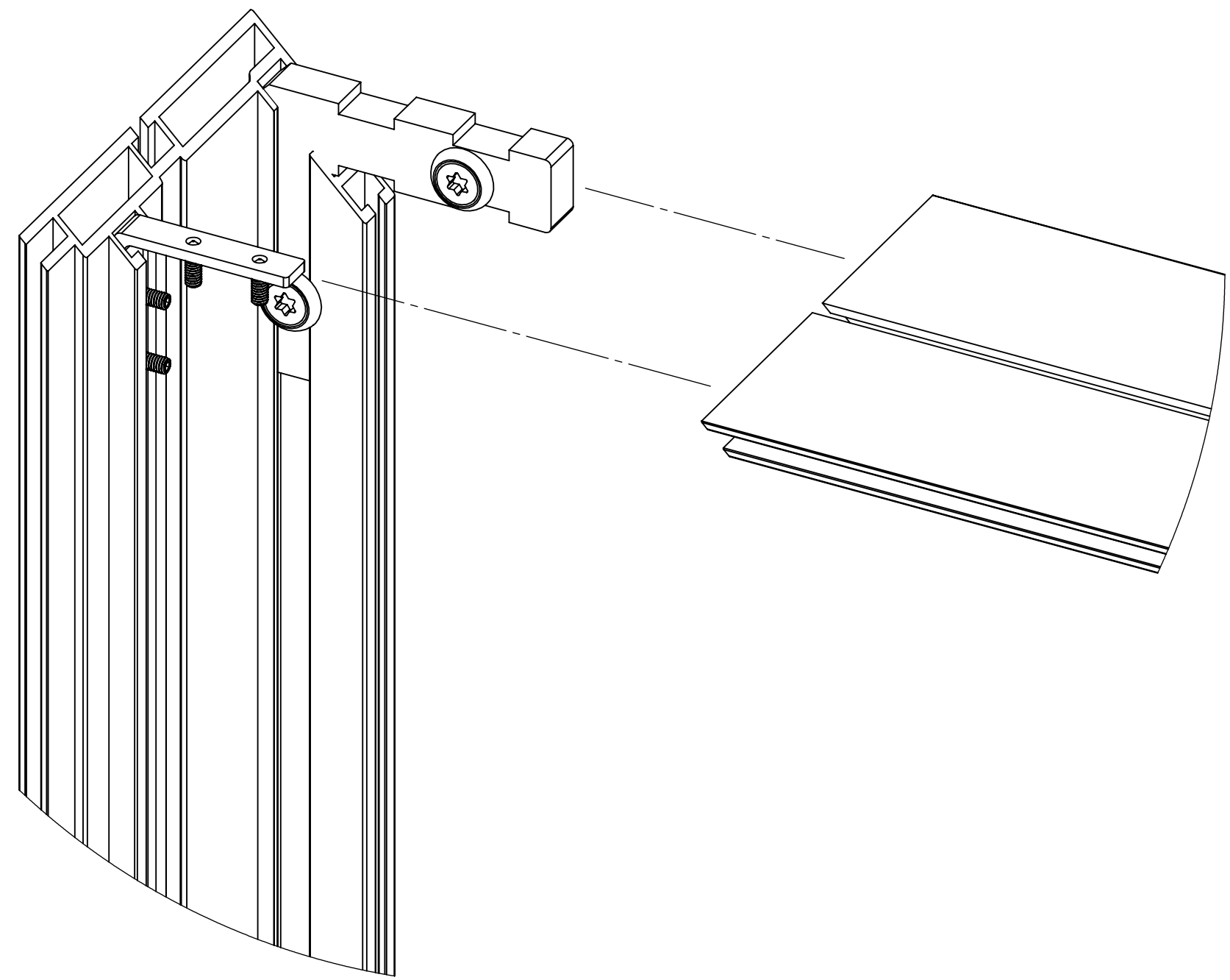
DETAIL A SCALE 3 : 4
